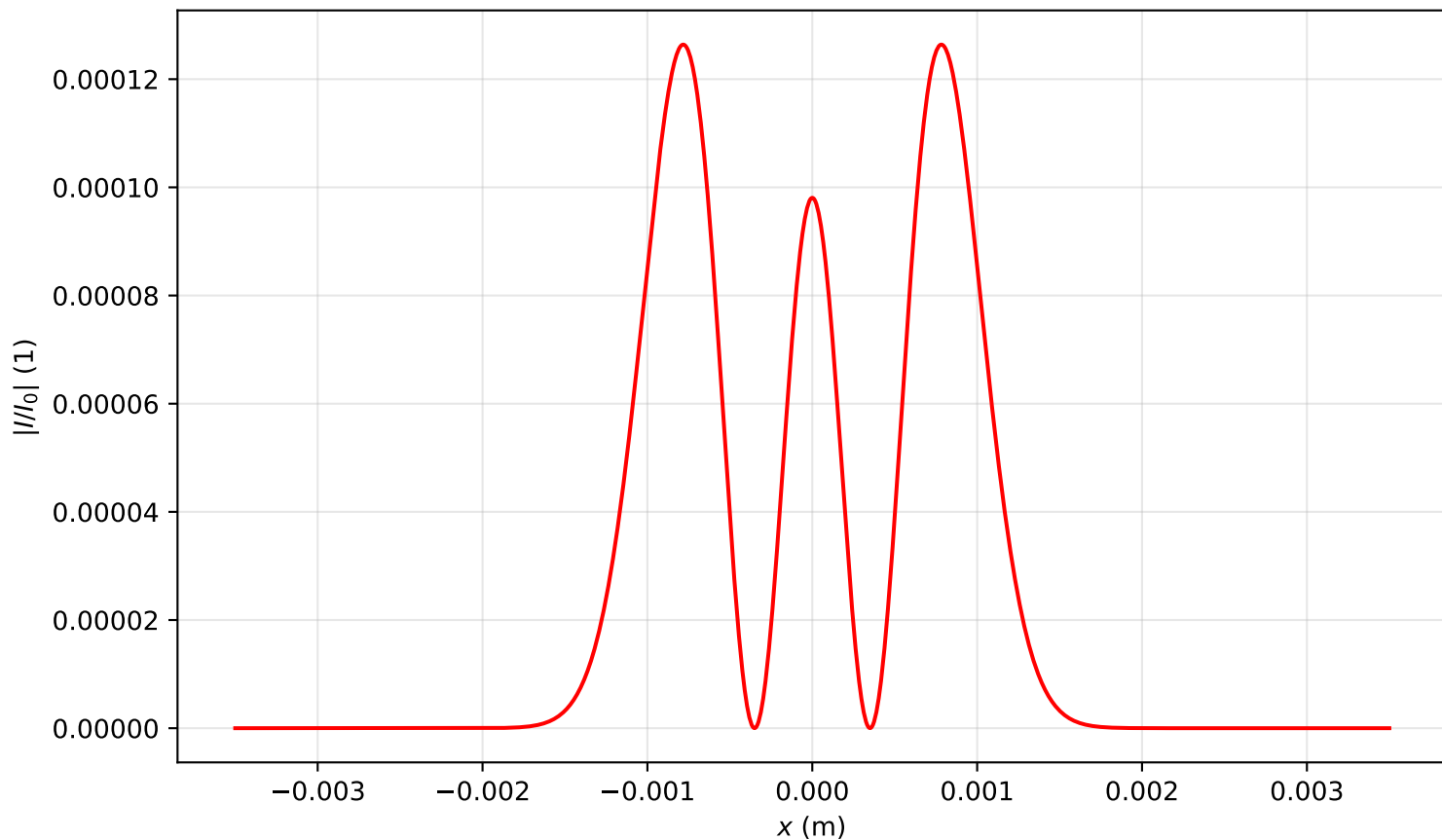
Intensity profile I(x, y = 0, z = 0.080)/I_0 , P_{in}=6.0P_{cr} , artificial time
